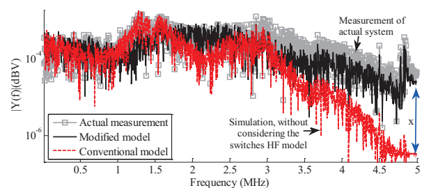
Fig. 25. Frequency spectrum of the common mode current.
