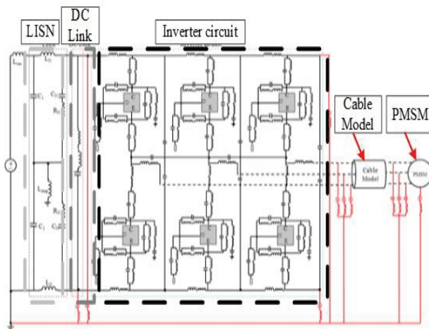
Fig. 22. Inverter circuit of AC motor drive, used in simulation with inclusion of parasitic components.
