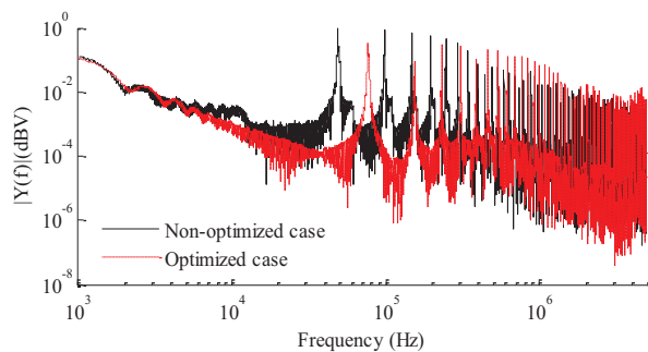
Fig. 31. Comparison of FFT spectrum between optimized and non-optimized quasi-resonant converter, resonant inductor’s current.
