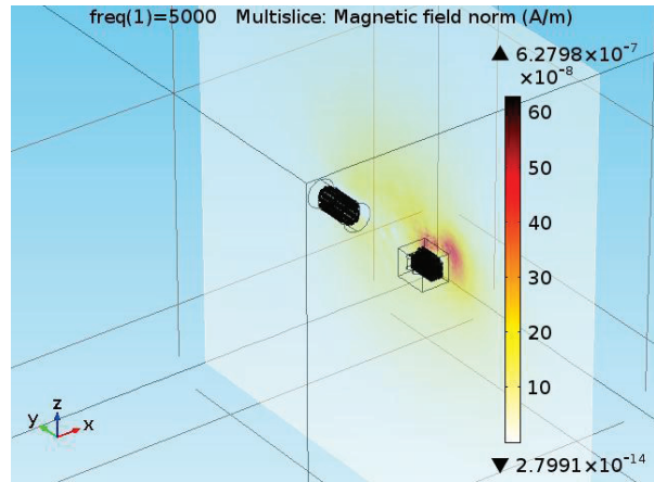
Fig. 16. Stray magnetic field intensity of the setup case 2 at 5 kHz simulated in FE ( \mu A/m ).
