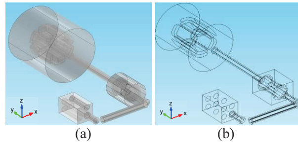
Fig. 5. Schematics of the power setup: (a) full FE model, and (b) equivalent model.
