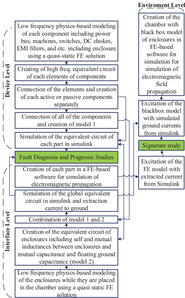
Fig. 2. Functional model of the numerical test environment.
