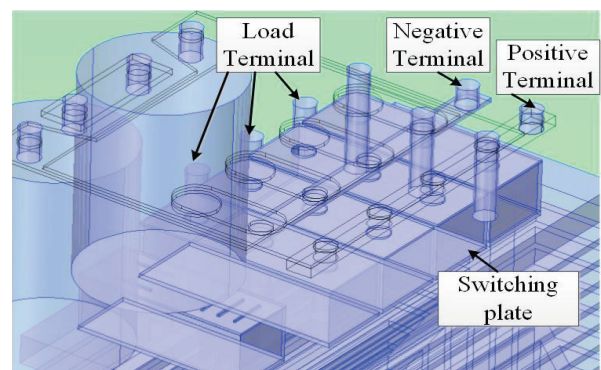
Fig. 12. Physical model of the inverter switches.
