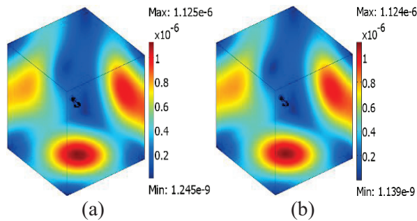
Fig. 6. Radiated magnetic flux density of: (a) 3D full model, and (b) wire model in Tesla (T).
