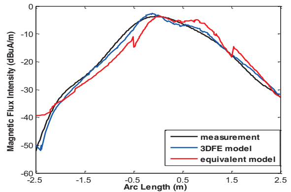
Fig. 8. The measured magnetic field intensity at 55 cm far from the setup on Y axis while all components were turned on at 60 Hz (dBμA/m).
