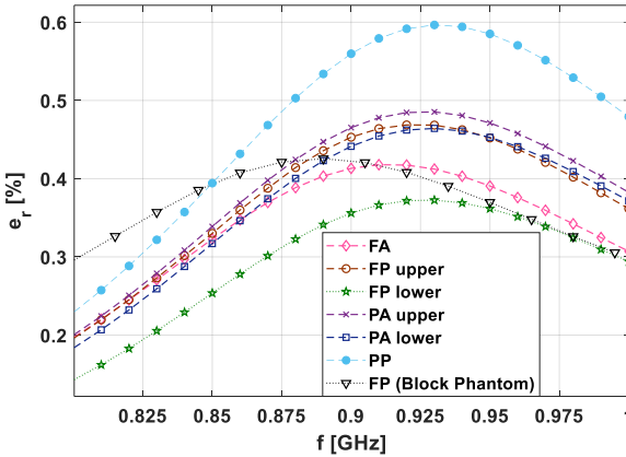
Fig. 4. Simulated antenna radiation efficiency in the semi-anatomical head model and the block phantom model.
