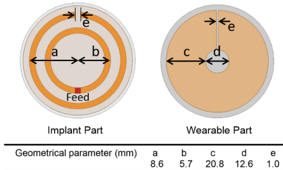
Fig. 1. Antenna system with its geometrical dimensions.
