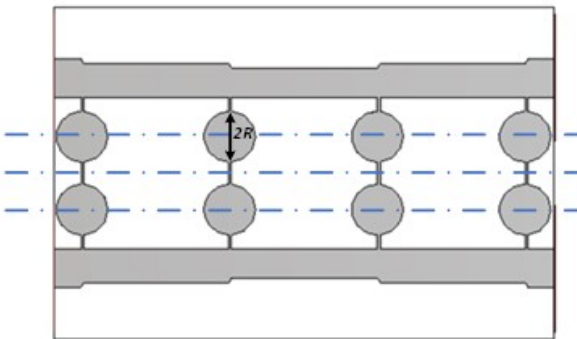
Fig. 7. Proposed UWB BLC with controllable coupling imbalance.
