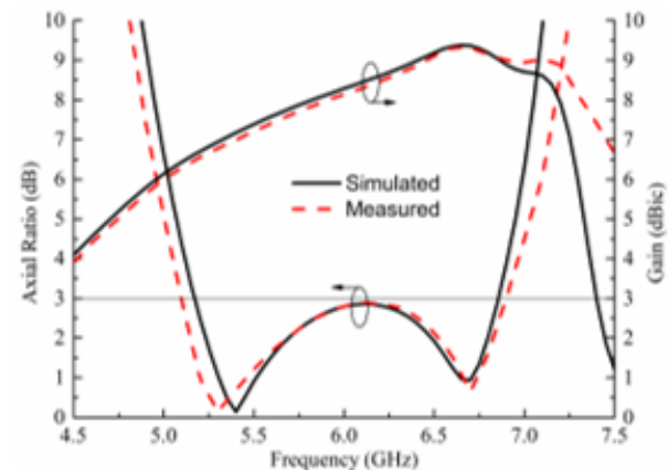
Fig. 10. Axial ratio and gain of the antenna.
