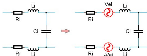
Fig. 5. Transformation of the elementary cell of equivalent circuit.
