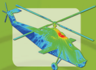
Antenna Placement
