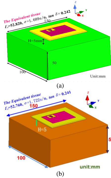
Fig. 8. The model of the proposed antenna and equivalent muscle tissue: (a) at the MBAN, and (b) at the ISM.
