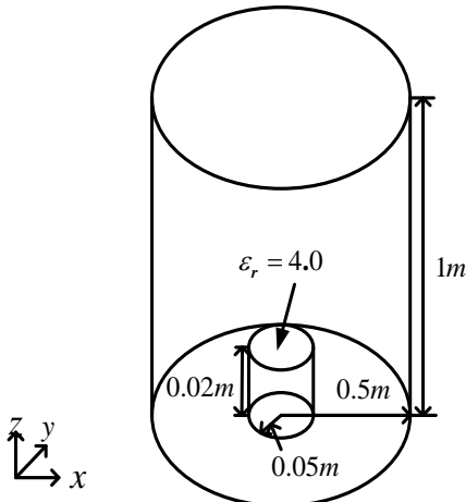
Fig. 3. A metal cylinder cavity loaded with a dielectric cylinder.
