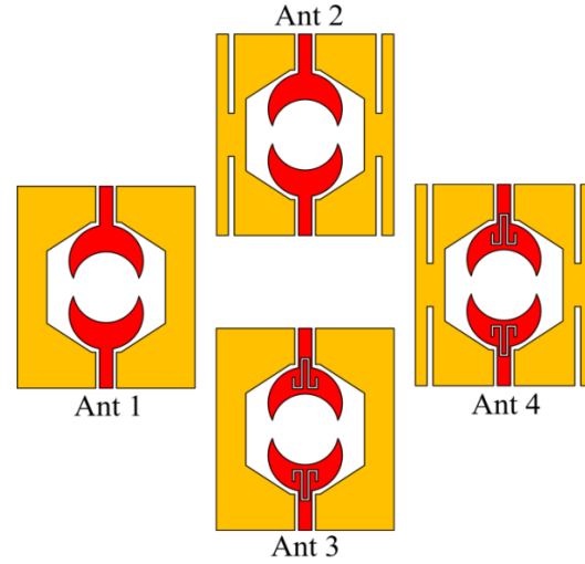
Fig. 2. Evolution of the proposed antenna.
