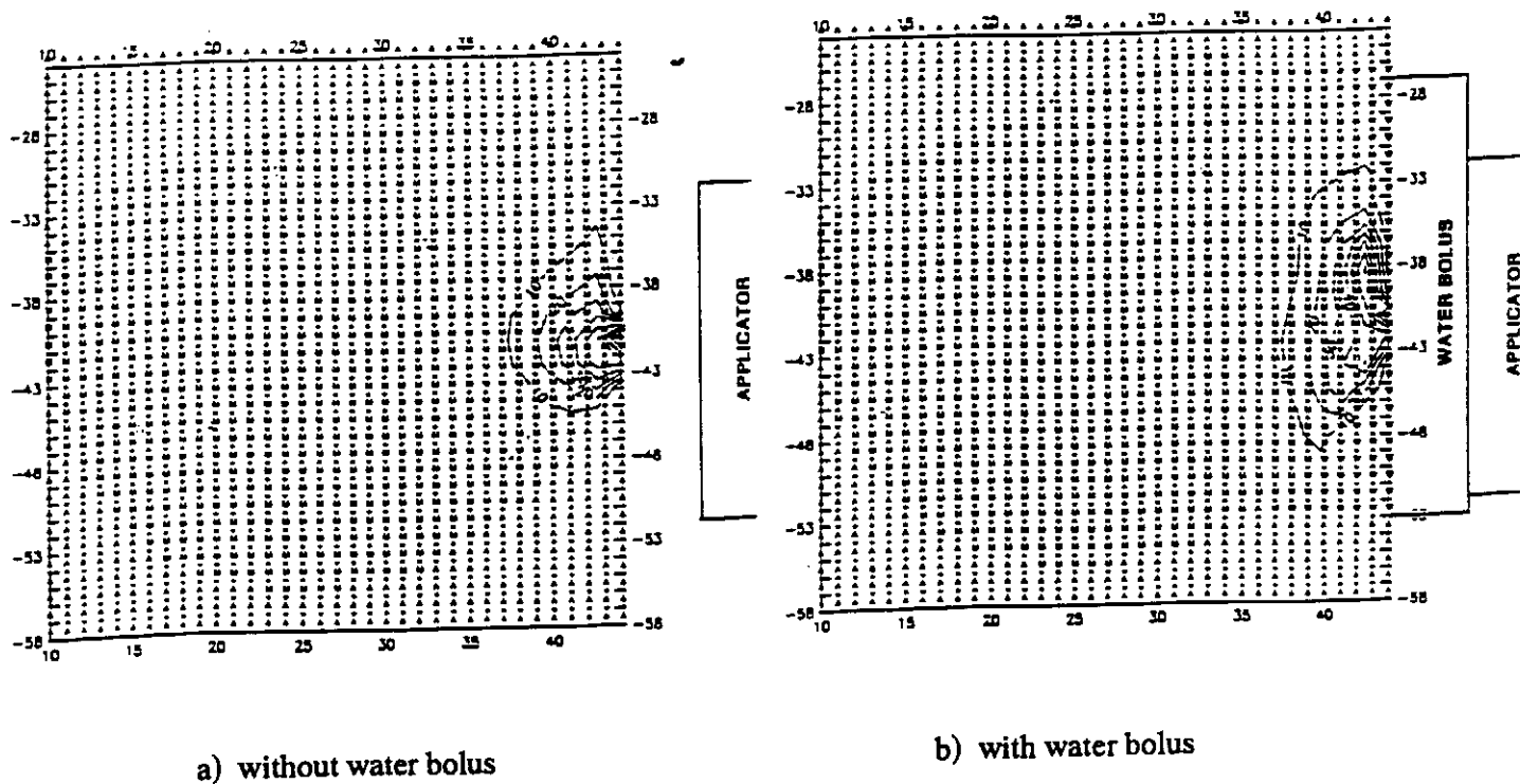
Figure 2. Normalized percent SAR distributions in a homogeneous thigh (M-Muscle, W-Water, A-Air)
