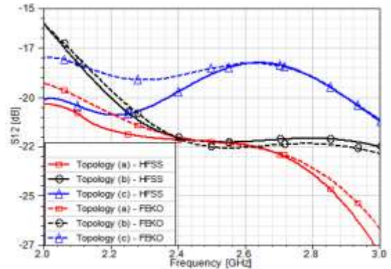
Fig. 3. E-plane patch orientation coupling for different U-slot topologies.
